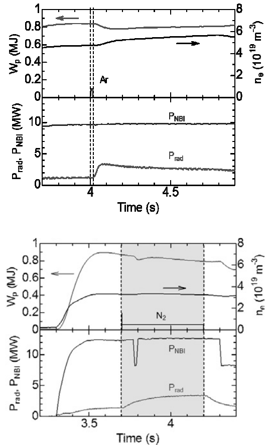
Fig. 1. Time evolutions of stored energy ( W_p ), line averaged density ( n_e ), NBI power ( P_{NBI} ) and total radiation power ( P_{rad} ) in typical Ar (top) and N 2 (bottom) seeded discharges, respectively.
