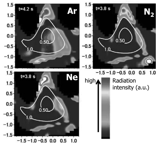
Fig. 2. Reconstructed radiation profile in Ar, Ne and N 2 seeded discharges, respectively, measured by AXUVD fan arrays 5) when P_{rad} reached maximum. Unit of horizontal and vertical axis is meter. White lines show 1/2\pi=0.5 and 1 surfaces.
