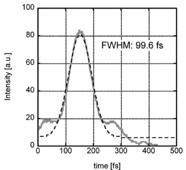
Fig. 3. The pulse shape of femto-second laser light measured by an autocorrelator. Dotted line is a Gaussian fitting calculation.
