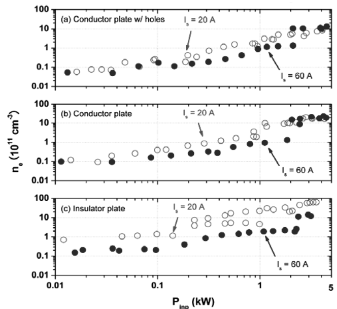
Fig. 1. Electron density n_e as a function of rf power P_{\text{inp}} , changing end plate material.
