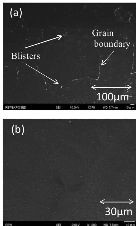
Fig. 1. (a) Autoradiograph of W exposed to D plasma (b) Autoradiograph of as received W
