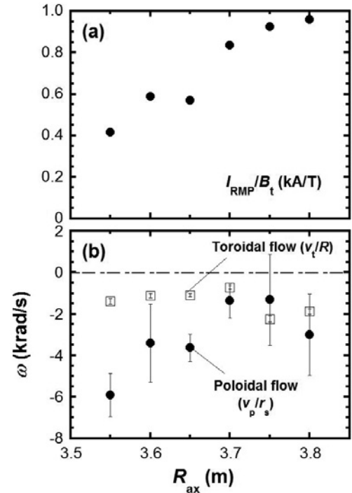
Fig.2 Changes of (a) threshold of mode penetration and (b) angular frequencies of toroidal and poloidal flows around \iota/2\pi = 1 resonance as a function of R_{ax} .
