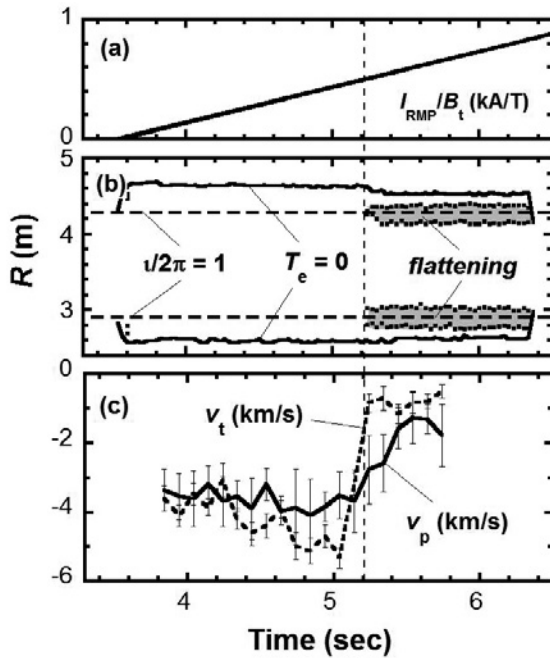
Fig.1 Time evolutions of (a) normalized RMP current and (b) plasma boundary, \iota/2\pi = 1 surface, T_e profile flattening and (c) toroidal and poloidal flow velocities around \iota/2\pi = 1 resonance.
