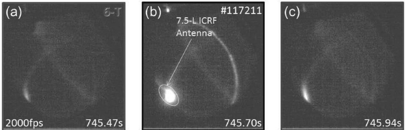
Fig. 1 Three snap shots of sparks occurred in the lower part of an ICRF antenna (7.5-L) observed with a fast framing camera installed in a tangential port (6-T) just before the termination of an ICRF heated long pulse discharge.
