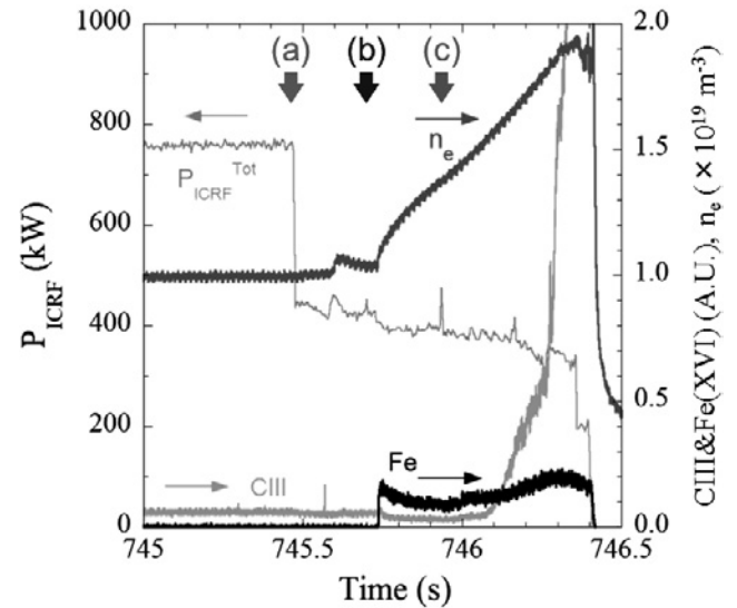
Fig. 2 Time evolutions of the total ICRF power, the plasma density and spectroscopic measurements (C and Fe) just before the plasma termination.
