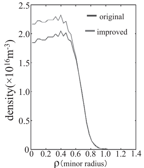
Fig. 2. Density distribution of the counter-injected particles.
