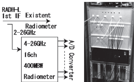
Fig. 1 A block diagram of 16ch cECE radiometer and a picture of the installed cECE radiometer system.
