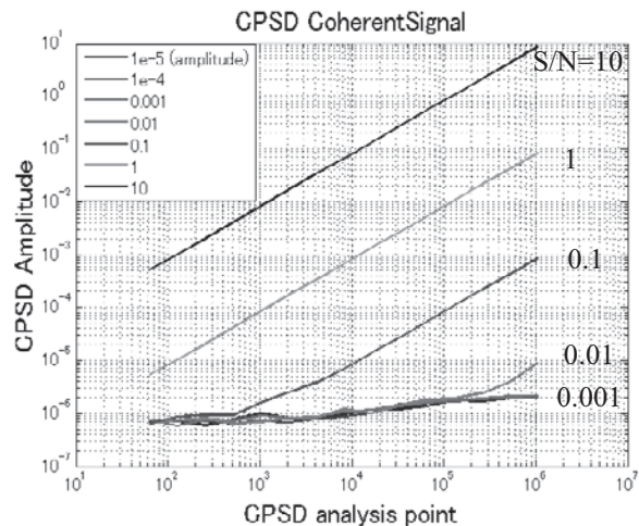
Fig. 3 Simulation results with sinusoidal signal type and the CPSD analysis.
