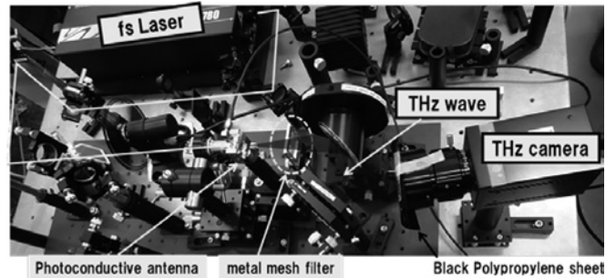
Fig. 1. Photograph of test system configuration. Femto-second laser light pumps up the THz wave at the photo-conductive antenna and it is led to THz camera.
