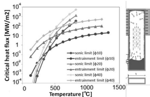
Fig. 4 Heat transfer characteristics for circular heat pipe.
