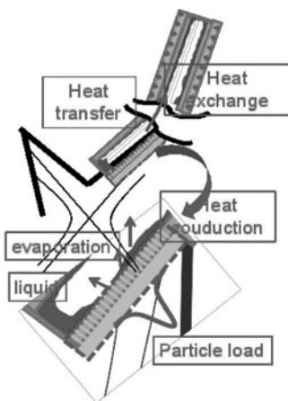
Fig. 1 Concept of the divertor component developed under this study.
