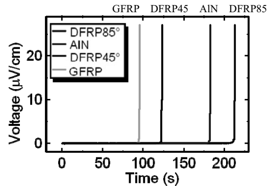
Fig. 2: Takeoff times of 4 coils. (Winding tension and coil current are respectively 10 N and 0.8I c .)
