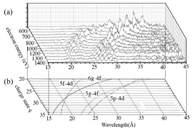
Figure 1 (a): Typical EUV spectra of highly charged tungsten ions obtained at electron energy E_e from 540 to 1370 eV in CoBIT. (b): The charge dependence of calculated wavelength.
