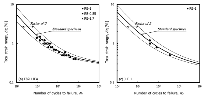
Fig. 1. Relationship between total strain range ( \Delta\epsilon_t ) and fatigue life ( N_f ) of the RB-0.85, RB-1, and RB-1.7 specimens of F82H-IEA, of the RB-1 specimen of JLF-1, and the regression curves of the standard specimen.
