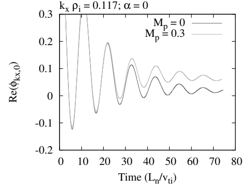
Fig. 1: Zonal flow response calculated by means of the flux-tube bundle model with and without poloidal rotation, where M_p denotes the poloidal Mach number of the \mathbf{E} \times \mathbf{B} flow 4) .
