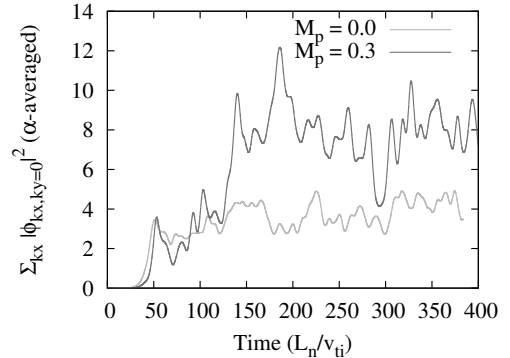
Fig. 2: Time-history of zonal flow potential driven by the ITG turbulence in a helical system with and without the poloidal \mathbf{E} \times \mathbf{B} rotation 4) .
