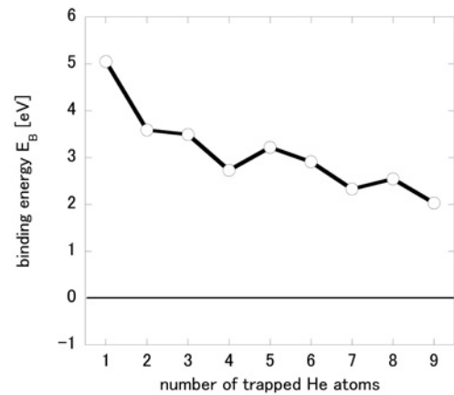
Fig. 1: Binding energy as function of the number of He atom trapped within a W monovacancy 2) .
