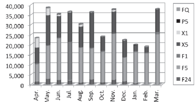
Fig. 1. CPU time (hours) used for each month in FY 2012.
