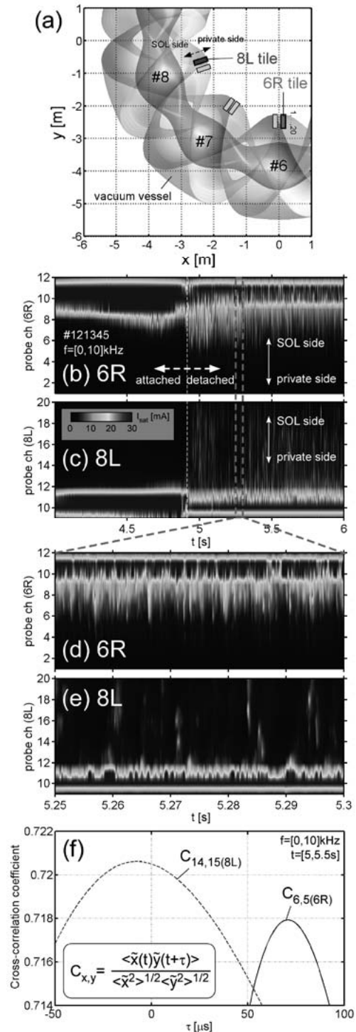
Fig. 1. Positional relationship of the divertor probe arrays (6R and 8L). (b) Contour plots of low-passed I_{\text{sat}} on 6R and (c) 8L divertor tiles. (d)(e) Magnified views of Figs. (b)(c). (f) Cross-correlation coefficients.
