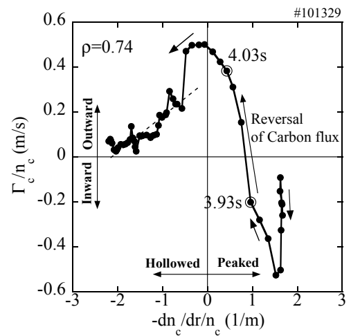
Fig. 2: Relation between flux of carbon normalized by the carbon density and gradient of carbon density normalized by the carbon density.
