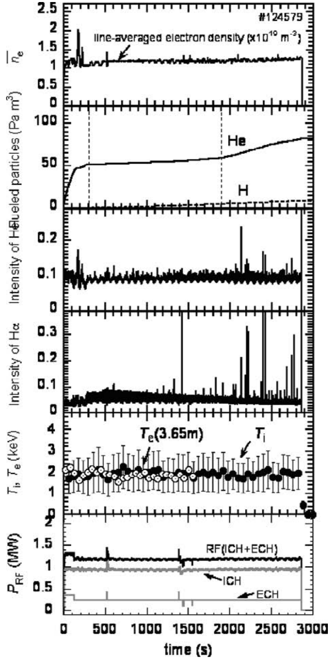
Fig.1 Discharge waveform in various plasma parameters in the 48 min discharge. Many plasma parameters were kept constant on the SSO.
