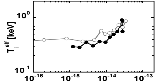
Fig.2 Variation of effective ion temperature with the increase of time integrated power of EGAM (\int_{t_0}^{t_0+\Delta t} (\delta B_\theta)^2 dt) . Open and closed symbols indicate variation of these values for particular EGAM events. The time duration of T_i^{\text{eff}} rise was chosen as \Delta t (see Fig.1).
