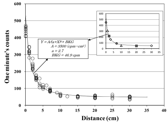
Fig.1 Dependence of one minute's counts on distance.
