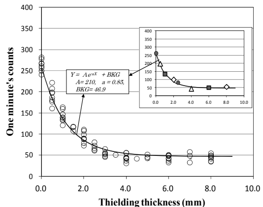
Fig.2 Dependence of one minute's counts on shielding thickness.
