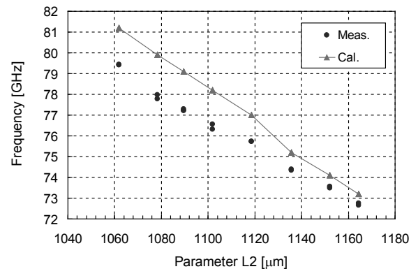
Fig. 2. Notch frequency as a function of pattern size.
