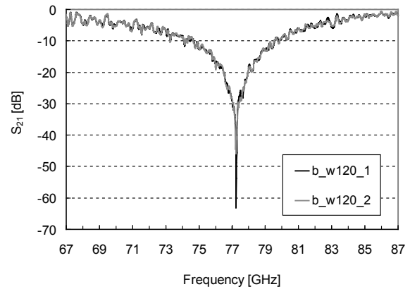
Fig. 1. Transmissivity ( S_{21} ) vs. frequency.
