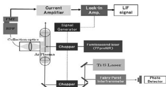
Fig.1 LIF system with an aid of femtosecond laser
