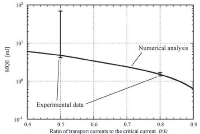
Fig. 1 MQE of MgB 2 transposed conductor.
