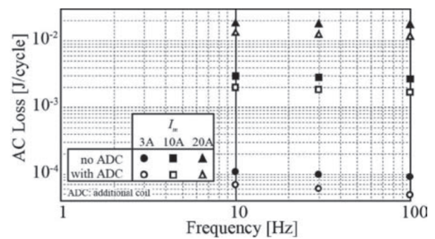
Fig. 2 AC losses in a sample coil with additional coils to suppress change of magnetic fields.
