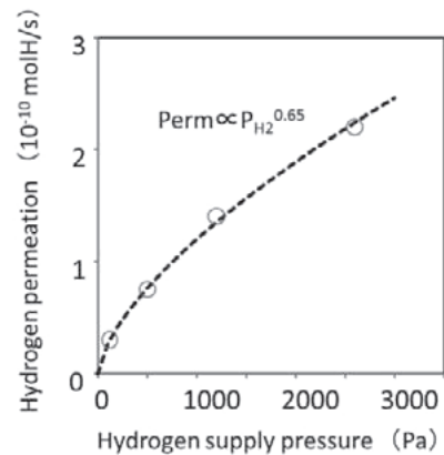
Fig. 3. Steady state hydrogen permeation through Ni/FLiNaK/Ni system at 823 K.
