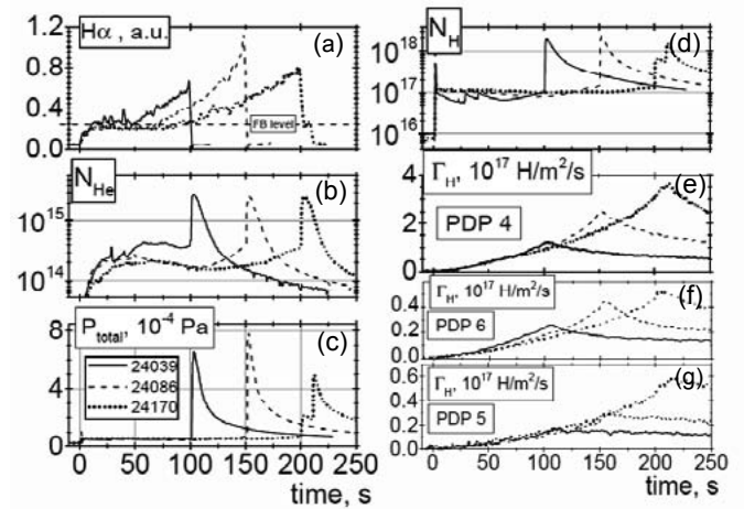
Fig. 2. Temporal evolutions of various parameters in the long pulse discharges. (a) H_{\alpha} intensity obtained by spectroscopic measurements, (b) number of He particles, (c) total pressure obtained with the ASDEX gauge, (d) number of hydrogen particles, (e), (f), (g) the atomic fluxes obtained with the PDP probes at bottom divertor, outboard side and top divertor, respectively.
