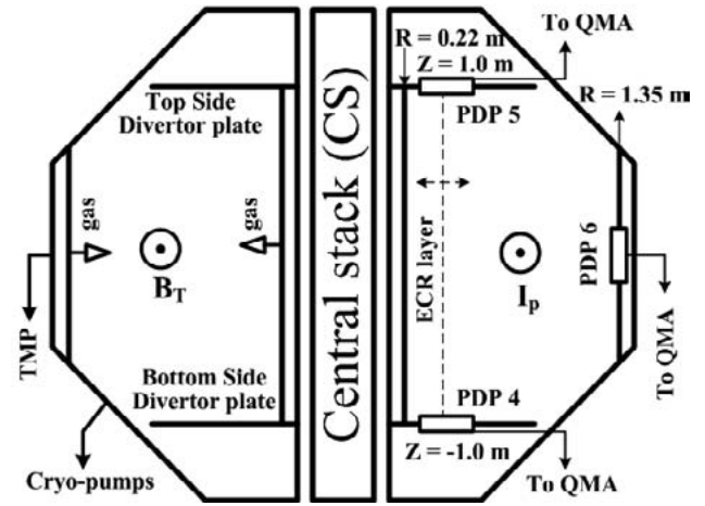
Fig. 1. The schematic of the QUEST tokamak with the location of the divertor plates (top and bottom) as well as the plasma driven permeation probes (PDP), direction of toroidal field, plasma current, pumping location, etc.
