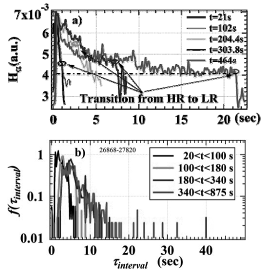
Fig.2 (a) H_\alpha transition at various time slices, (b) time dependent probability function of \tau_{interval}
