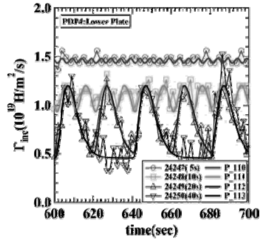
Fig.1 Incident H -fluxes at various puff intervals (5s to 40sec). Symbols are experimental data and solid curves are numerical ones.
