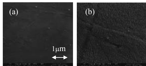
Figure 2 Surface morphologies of F82H measured by FE-SEM. (a) deuterium bombardment and (b) helium pre-irradiation and deuterium bombardment.
