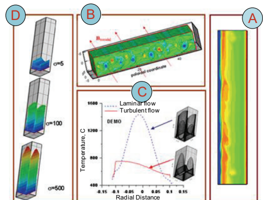
Fig. 2. A: MHD buoyancy flow B: MHD Q2D flow C: MHD turbulent effect on temp. profile D: M-shaped velocity profile
