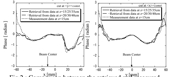
Fig. 2 : Comparison between the retrieved and measured phase profiles
