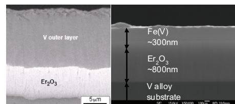
Fig. 1 Double layer of \text{Er}_2\text{O}_3/\text{V} and \text{Er}_2\text{O}_3/\text{Fe} on V alloy
