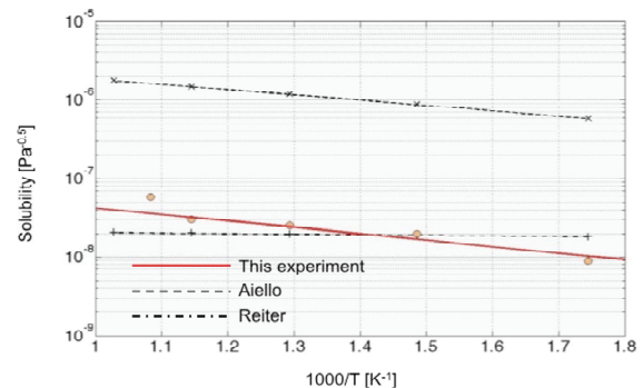
Fig. 1 Temperature dependence of hydrogen solubility in LLE (initial results)
