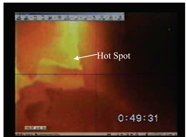
Fig. 1 In-situ observation of hot spot in a ferrite sample exposed to H- field in 2.45 GHz 5 seconds after microwave turned on, the brightest spot exceed 1200 degree C, the dark part was less than 800 degree C. The scale is 100 micron. Temperature gradient was estimated to a few thousands degree C / 1 mm.
