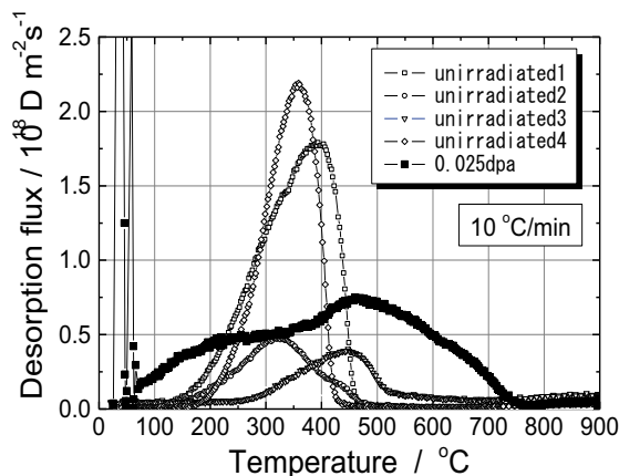
Fig. 1. Preliminary data on deuterium desorption from W sample irradiated by neutron at 50 °C for 0.025 dpa. Spectra from unirradiated tungsten samples are also shown.
