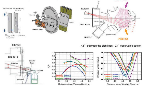
Fig. 1 (left upper) the main part and the movable stage, Fig. 2 (left lower) the vertical sight lines, Fig. 3 (right upper) the horizontal sight lines, Fig. 4 (right lower) (left) the pitch angle, (right) the equivalent radius.
