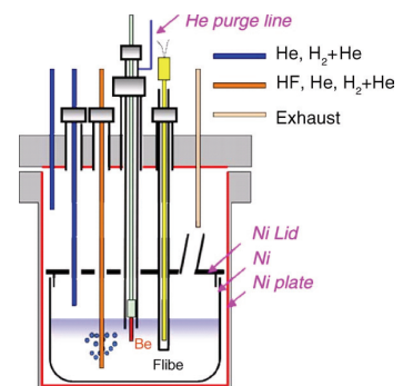
Fig. 1 Reactor for measuring redox
