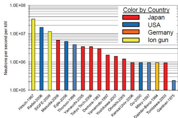
Fig.2 Neutron production rate of IEC devices 1)
