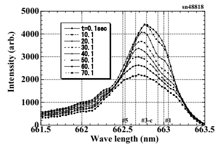
Fig.2 Temporal profile for full energy beam component for 74 s long pulse injection(sn48818). V_{full}=95 kV, I_{acc}=14 A(IS-2B).
