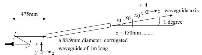
Fig. 1: Experimental setup the principle experiments for beam coupling and mode content analysis
