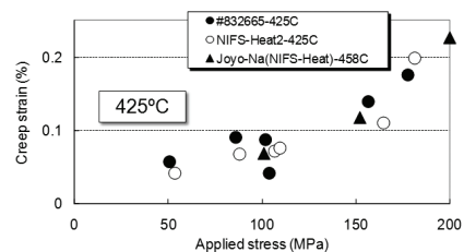
Fig. 2 Creep strain vs. applied stress for US832665 and NIFS-Heat 2 in HFIR Li capsule and Joyo Na-capsule
