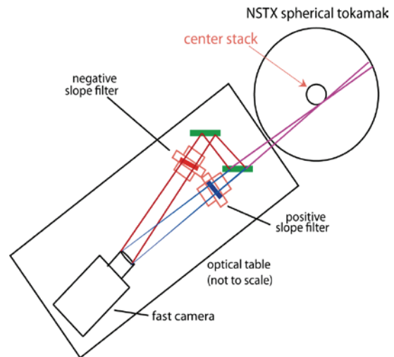
Fig. 2. Proto-type of SWIFT installed in NSTX
