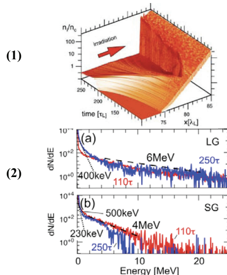
Fig.2 (1) time dependent density profile of plasmas interacting with pico second heating pulse, (2) electron energy spectrum for long scale (a) and short scale cases
