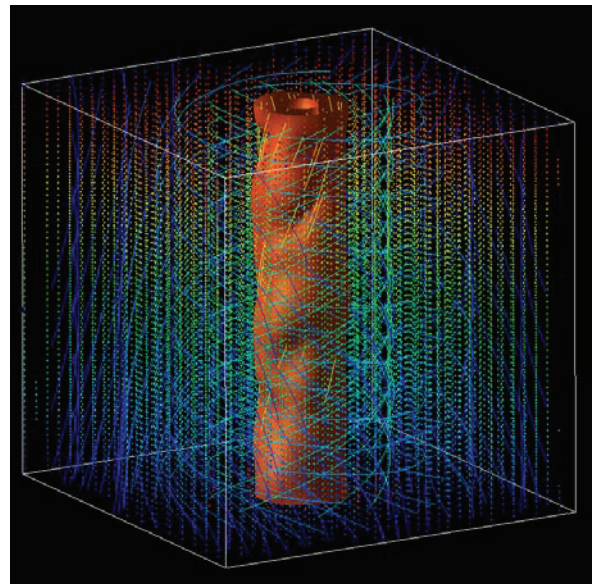
Fig.2: Test particle simulations with a vortex.
