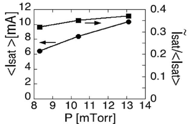
Fig. 2 The averaged value of I_{\text{sat}} and fluctuation level as a function of neutral pressure P .
