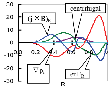
Fig. 2. Ion fluid force balance: pressure gradient force (red), Lorentz force (blue), electric force (green) and centrifugal force (purple).
