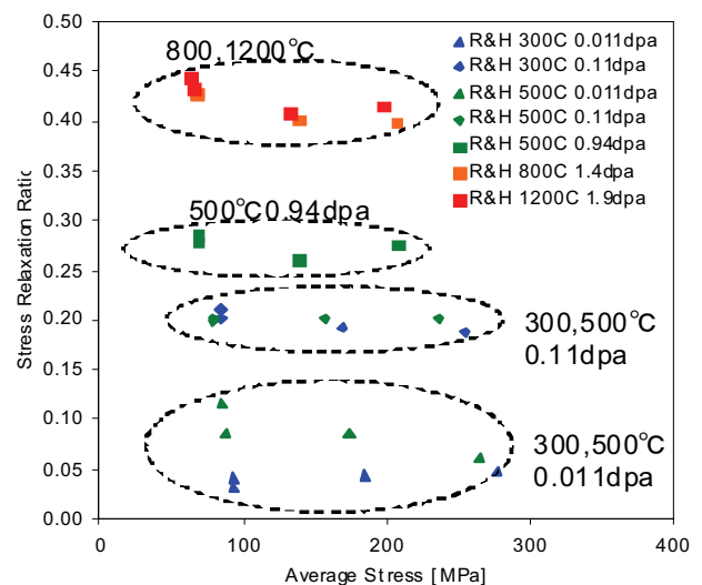
Fig.1 Stress Relaxation Behavior of CVD-SiC after HFIR Irradiation
