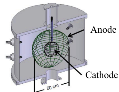
Fig.1 Schematic view of IEC device 1)
