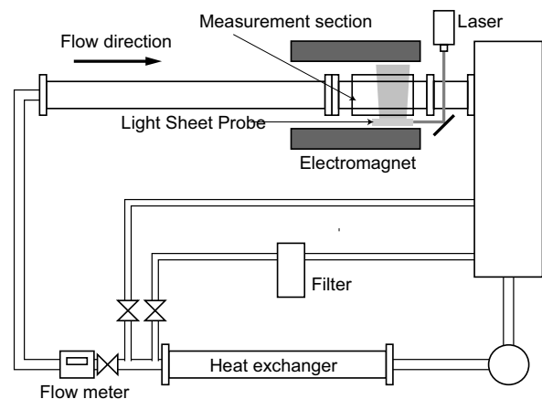
Fig. 1 Schematic drawing of FLiHy facility
