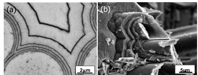
Fig. 1 A SEM image of (a) multilayer (C/SiC) fiber/matrix interphase and (b) fracture surface of the composites
