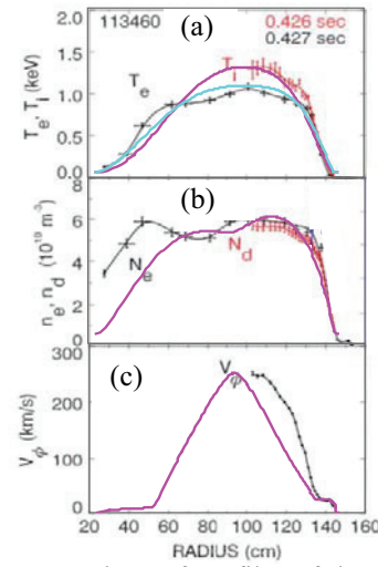
Fig. 1. Comparison of profiles of the computed equilibrium with NSTX shot 113460 (see Fig.2 of Ref.3): a) computed ion (pink) and electron (cyan) temperatures; b) computed density (pink); c) computed ion toroidal flow velocity (pink).
