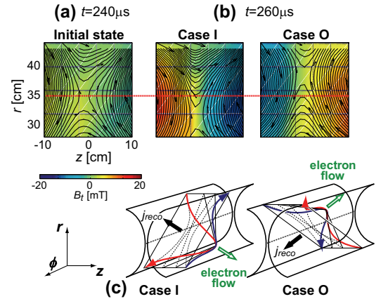
Fig. 2. Poloidal magnetic flux contours (solid lines) with poloidal magnetic field (arrows) and toroidal magnetic field (color coded) at t=240 \mu\text{s} (a) and at t=260 \mu\text{s} (b) in cases I (left) and O (right) counter-helicity merging, and corresponding three-dimensional illustrations of reconnecting field lines in the Hall-MHD regime (c) [2].
