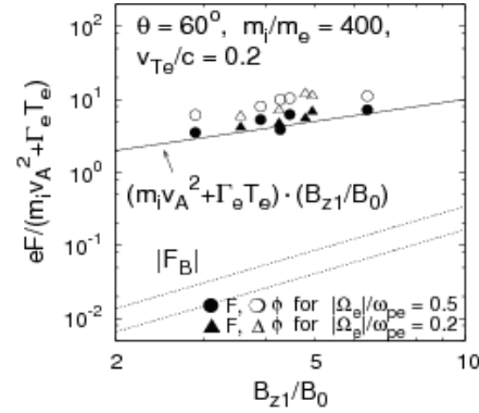
Fig. 1 Parallel pseudo potential F versus shock amplitude. The closed circles and triangles show F while the open ones represent electric potential formed in shock waves [2].
