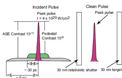
Fig. 1: Schematic of the relativistic plasma shutter for ultra intense laser pulses.
