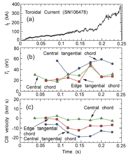
Fig. 2. Time evolution of the toroidal current (a), Doppler ion temperature (b) and CHI ion flow velocity (c).
