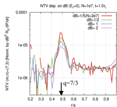
Fig.1 : An example of NTV calculation on tokamak with small perturbation magnetic field. On the q=7/3 surface where the perturbation field resonates with background magnetic field, peaking of NTV is found. And the magnitude of NTV is found to be proportional to the square of the magnitude of field perturbation, \delta B^2 .
