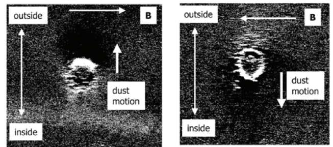
Fig. 2 Dust transport depending on direction of magnetic field.
