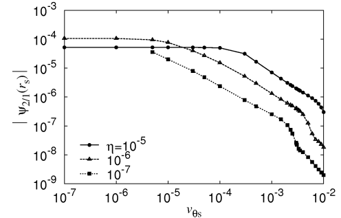
Fig.1. Magnetic flux of the penetrated error field |\psi_{2/1}(r_s)| versus the rotation velocity at the rational surface.
