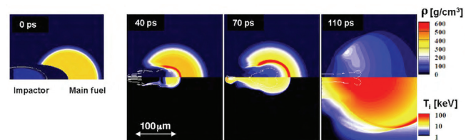
Fig. 2. Snapshots of density and temperature distributions obtained from the two-dimensional simulation. At t = 110 ps, ignition and burn can be observed with temperatures > 30 keV.
