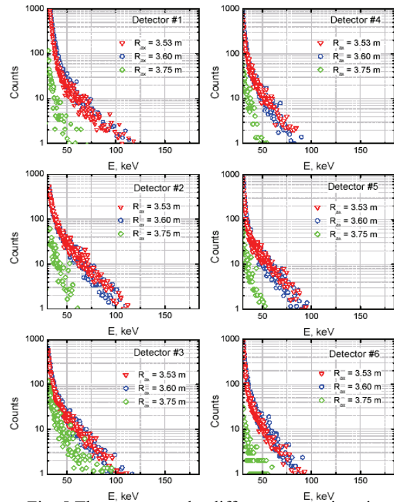
Fig. 5 The spectra at the different magnetic axis.
