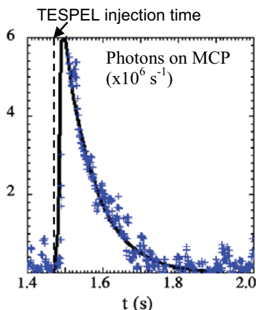
Fig. 1. Background subtracted 45.5 \text{ \AA} signal (+) and MIST simulation assuming 7 \times 10^{17} Mg atoms injected at r/a < 0.7 and 1.5 \text{ m}^2/\text{s} constant diffusivity [from Ref. 2].
