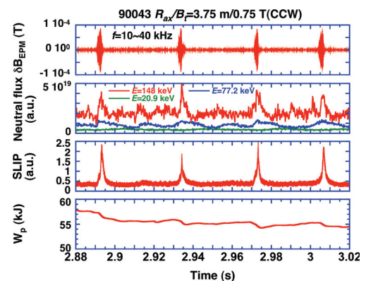
Fig. 2. Time traces of \delta B_{EPM} at the Mirnov coil position, charge exchange fast neutrals for three different particle energies, beam-ion loss rate to SLIP ( E \sim 160 \text{ keV} , \chi \sim 30 \text{ deg.} ) and W_p .
