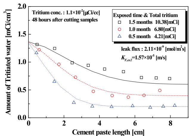
Fig. 1 Comparison of observed values and estimated values for the distribution profile of tritium in concrete.
