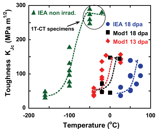
Fig. 1. Temperature dependence of fracture toughness of F82H specimens irradiated to 18 dpa. Results indicate substantial reduction of the effect of radiation on fracture toughness due to optimization/tightening of tempering conditions. Miniaturized bend bar specimens were used. Data shown in the circle were measured from large size (1T-CT:1 inch thickness) specimens.
