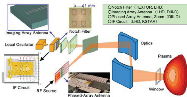
Fig. 1. Configuration of microwave imaging system.
