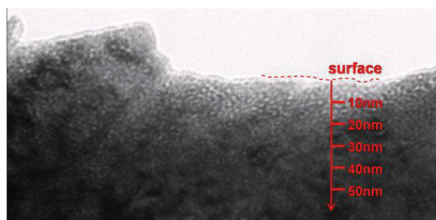
Fig. 1 Cross sectional view of He nano bubble layer exposed to D/He mixed plasma at 573 K.
