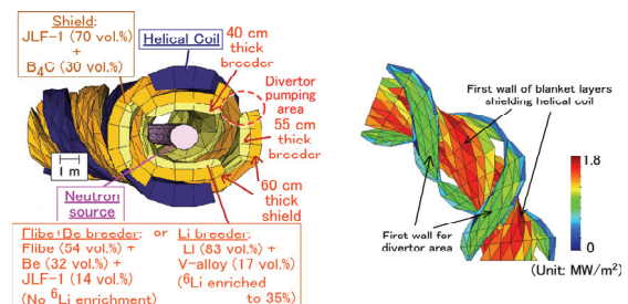
Fig. 1 Example of 3-D geometry data with MCNP (~3,000 cells) and helical neutron wall loading
