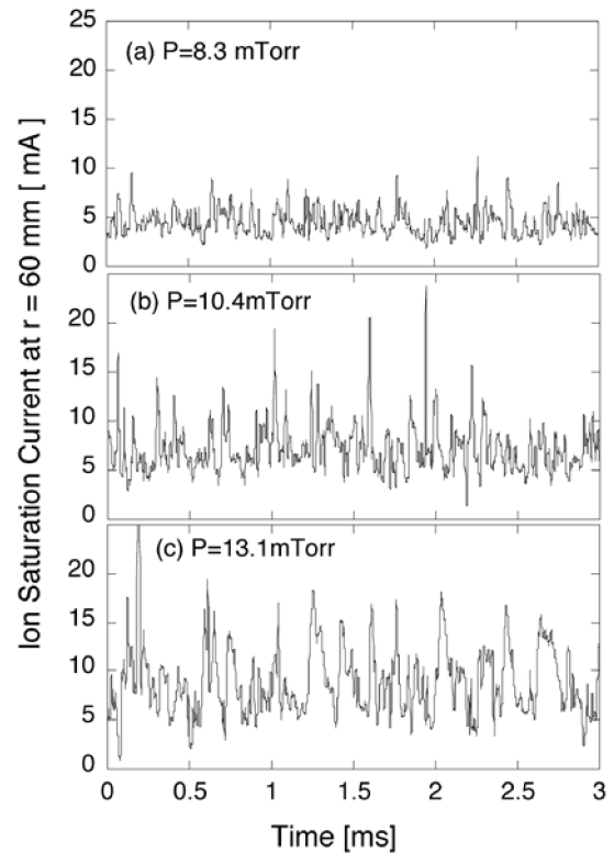
Fig. 1 Neutral pressure dependence of time evolution of I_{\text{sat}} at r = 60 \text{ mm} .
