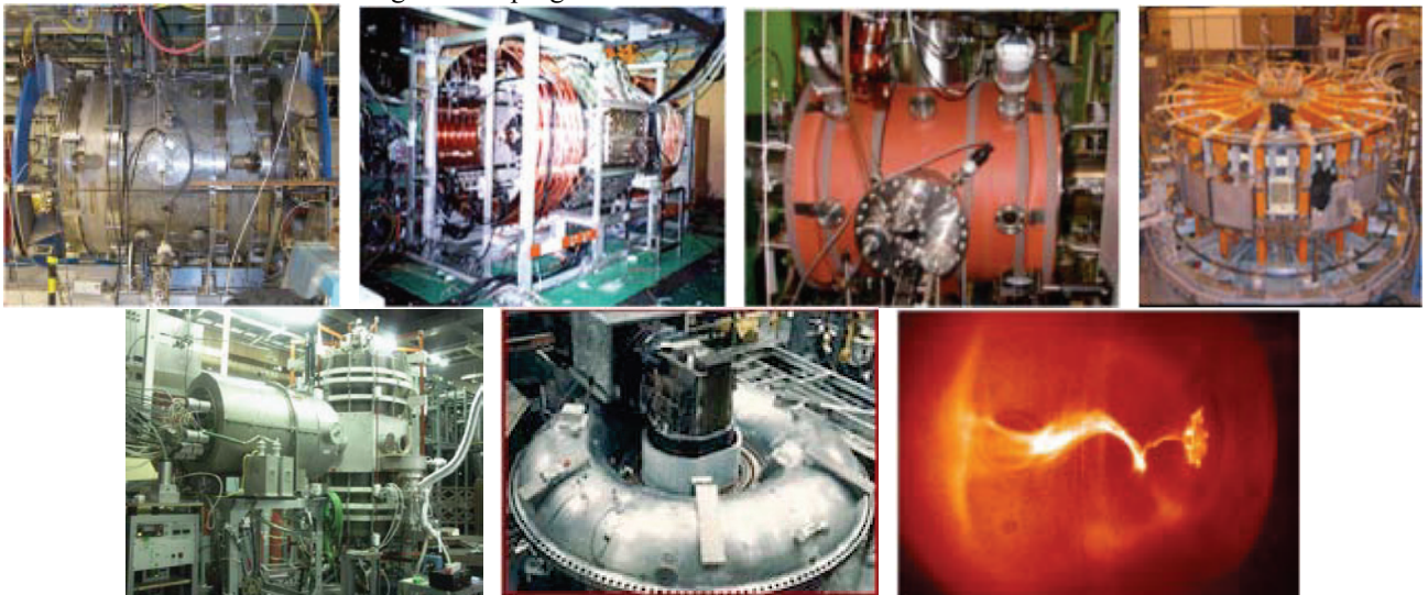
Fig. 1: Laboratory Experiments of Magnetic Reconnection: MRX (Princeton Univ.), TS-4 (Univ. Tokyo), SSX (Swarthmore College), VTF (MIT), UTST (Univ. Tokyo), MST (Univ. Wisconsin), Reconnection Exp. (Caltech)
