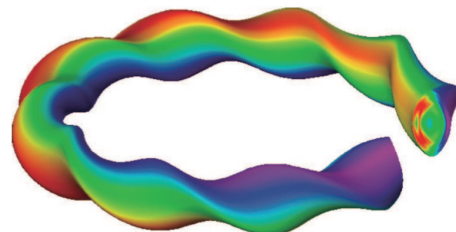
Fig.2. Three-dimensional eigenmode structure for a TAE mode in LHD 3) .
