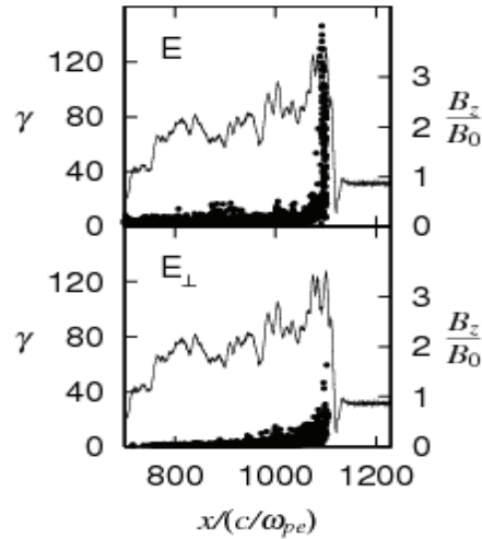
Fig. 2 Phase spaces ( x, \gamma ) of test electrons. The upper and lower panels, respectively, show test electrons calculated with total and perpendicular electric fields. There are many ultrarelativistic ( \gamma > 100 ) electrons in the upper panel [1].
