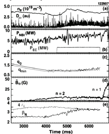
Fig. 2. Evolution of plasma behavior of a preemptive ECCD discharge in DIII-D. (a) line-averaged density and D_{\alpha} emission, (b) EC wave power and time-averaged neutral beam power, (c) central and minimum value of safety factor, (d) amplitudes of n = 2 and n = 1 tearing modes and (e) normalized beta and four times the internal inductance (an estimate of the beta limit for the ideal n = 1 kink mode in the absence of a conducting wall). [from Ref. 7]
