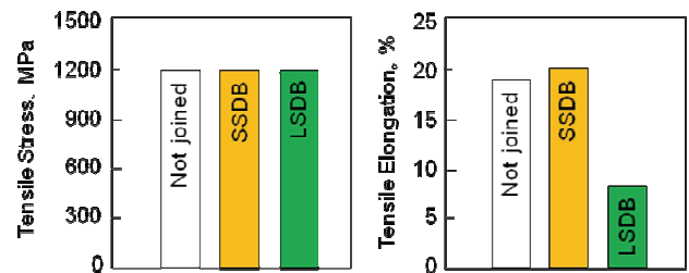
Fig.2 : Tensile stress and elongation of the ODS steel with and without joining.
