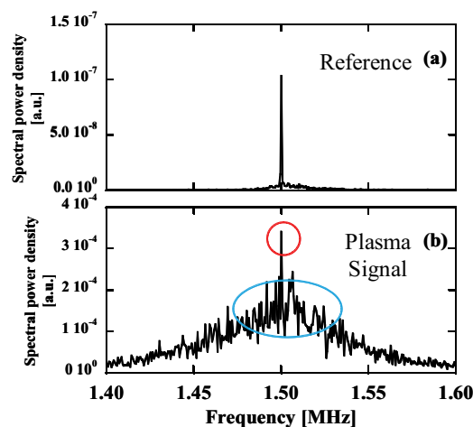
Fig. 1. Power spectrum of the reference signal (a) and that of the plasma signal of the heterodyne microwave reflectometer, during the HHFW heating in NSTX.
