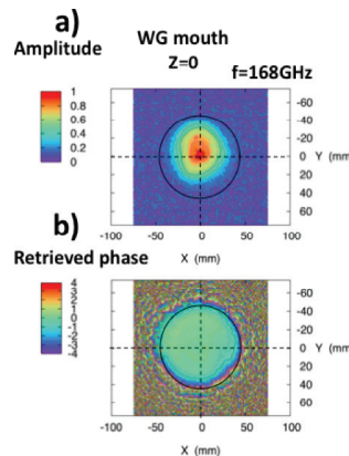
Fig. 3 : a) Measured amplitude profile and b) retrieved phase profile
