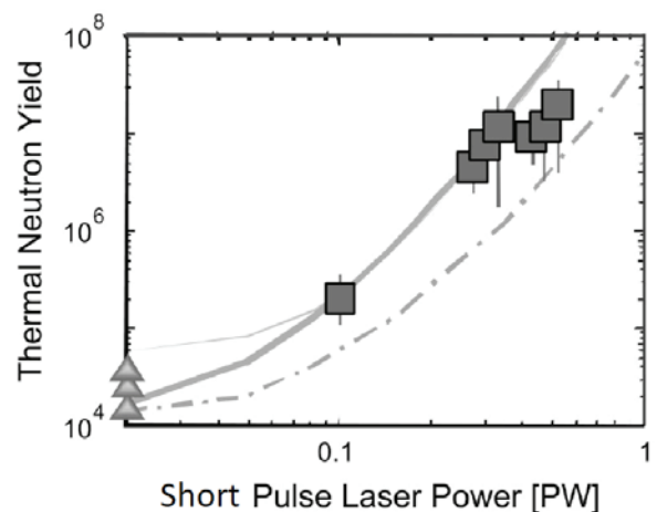
FIG.2. Neutron number vs fast heating laser power. The triangles show the data without fast heating. The squares show the data with fast heating. The neutron increase is 1000 times with the heating compared to the ones without it. The fitted curves are the ones with 30% and 15% coupling efficiencies from the ultra-intense laser to the core heated energy.
