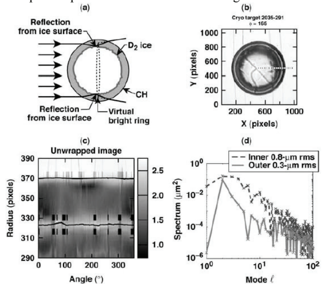
Fig. 2 Quality of solid Dr layer for cone-less fast ignition target at Rochester University
