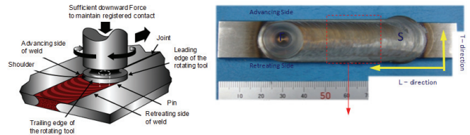
Fig.1 : Schematic diagram of FSW method and a FSW treated ODS steel.
